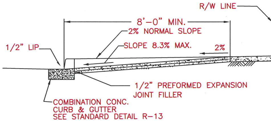
SECTION B-B TANGENT LOCATION
